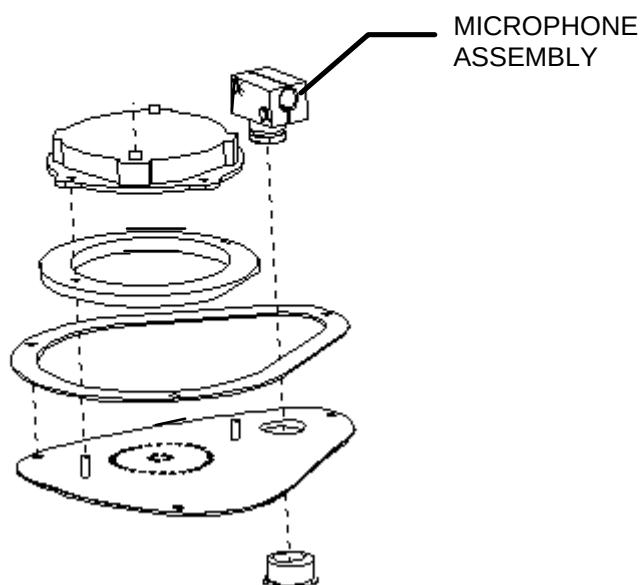
SPEAKER/MICROPHONE ASSEMBLY DETAIL ILLUSTRATION 1-2
