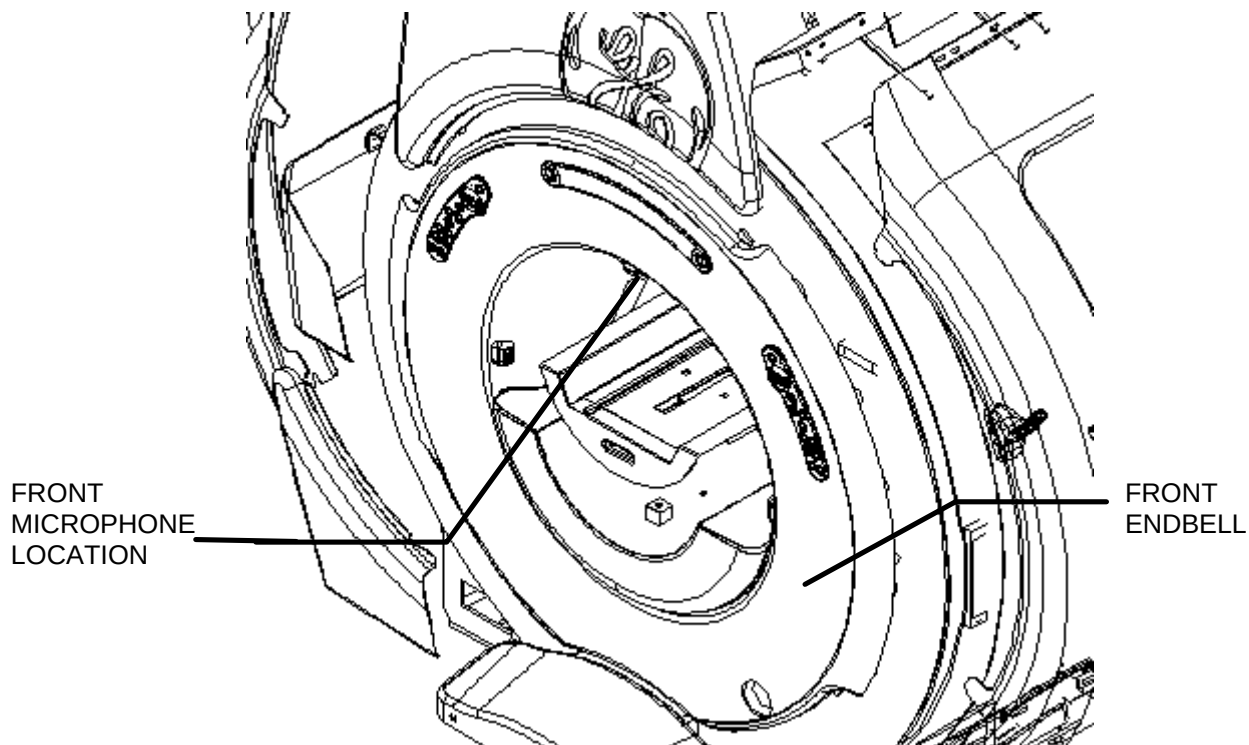
FRONT END BELL ILLUSTRATION 1-4
