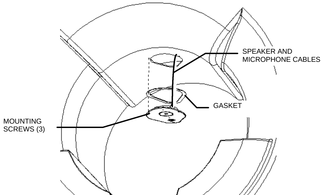
REAR VIEW OF MAGNET ILLUSTRATION 1-1
